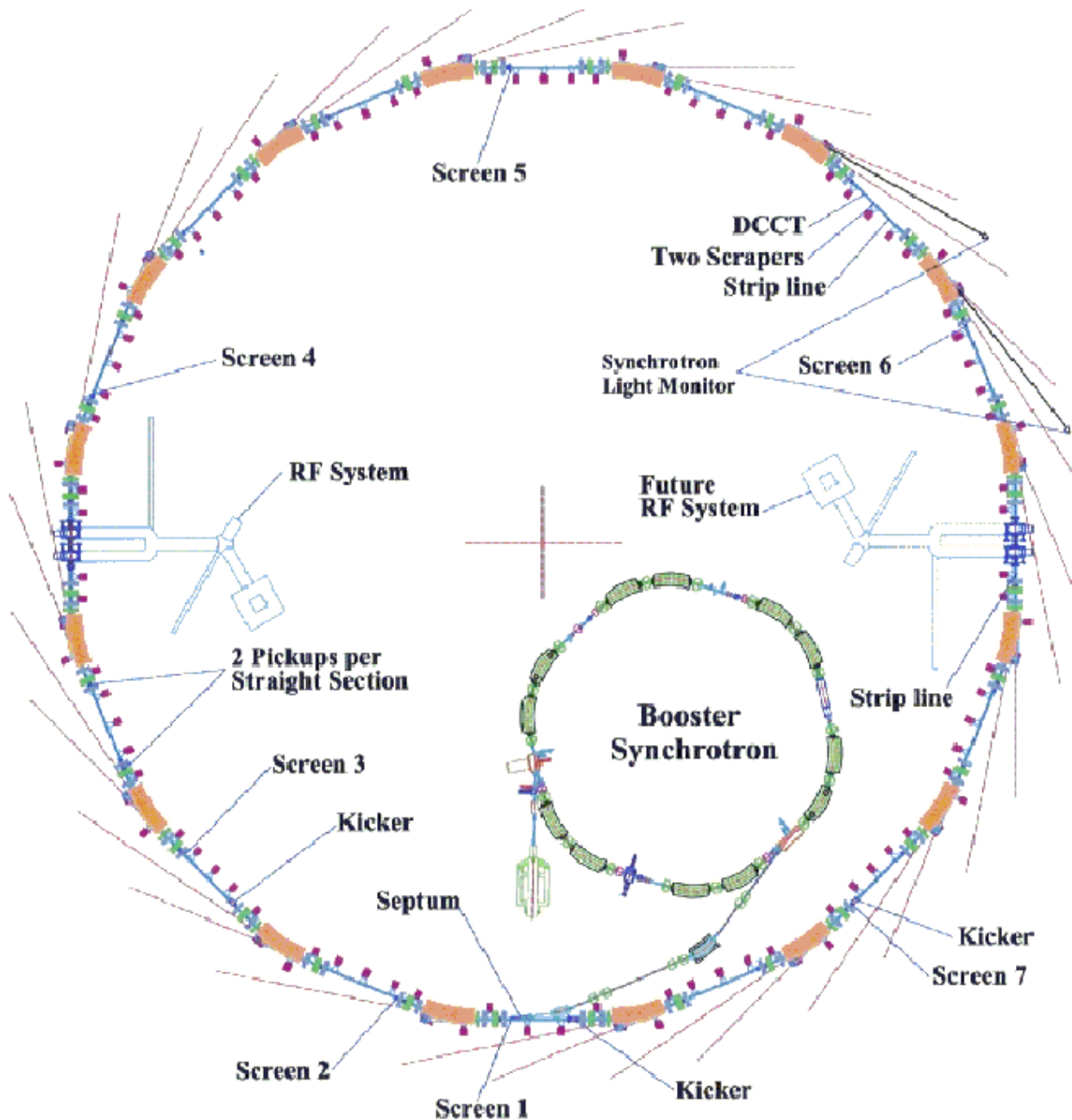
Figure 10.1: The layout of the storage ring SESAME with the proposed diagnostic elements
