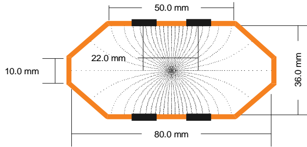
Figure10.2: Beam position monitor and the field created by a centered beam
