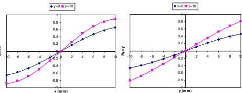
Figure 5: bpm sensitivity curves for x-direction (left) and y-direction (right).
