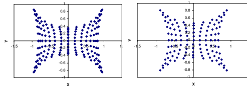
Figure 4: Position map with 30 mm (left) and 24 mm (right) H distance. distance between dots is 2mm.
