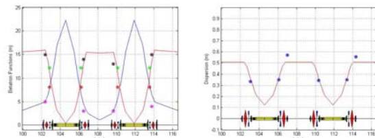
Figure 8: (Left) measured \beta_x (black) and (green), \beta_y (pink) and (red) at QF and QD respectively compared to theoretical ones in red and blue. (Right) measured dispersion (blue) compared to the theoretical one (red).
