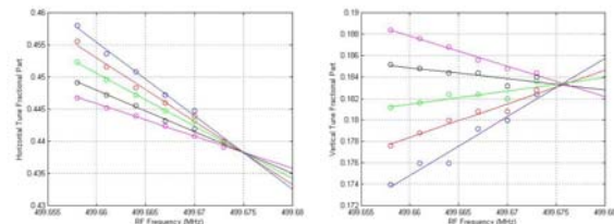
Figure 7: Chromaticity curves showing central RF frequency in the storage ring at 800 MeV.
