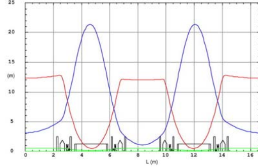
Figure 1: Optics 1 of SESAME storage ring showing betatrons \beta_x (red), \beta_y (blue) and dispersion \eta_x (green).
