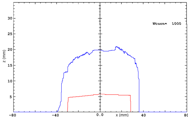
Figure 4: On-momentum dynamic aperture (blue) and vacuum chamber limited one (red) in the middle of the Long straight section, taking in account the effect of all the high order multipoles in the magnets.
