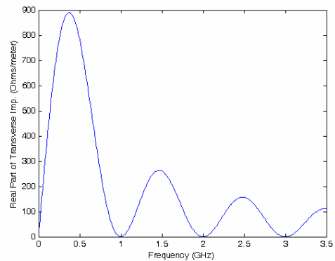
Figure 6: Real part of transverse impedance vs. frequency.
