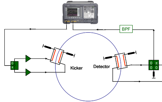
Figure 1: Simplified block diagram for tune measurement.
