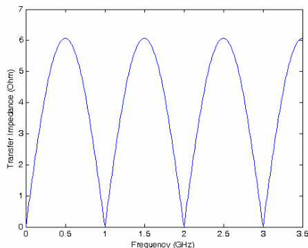
Figure 4: Stripline frequency response
