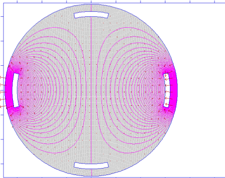
Figure 3: Full cross section of the stripline and EM field lines.
