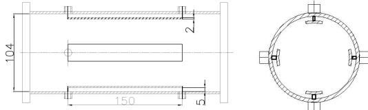
Figure 2: Schematic of stripline side view and cross section.
