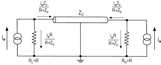
Figure. 7: Equivalent circuit for the stripline as a transmission line.
