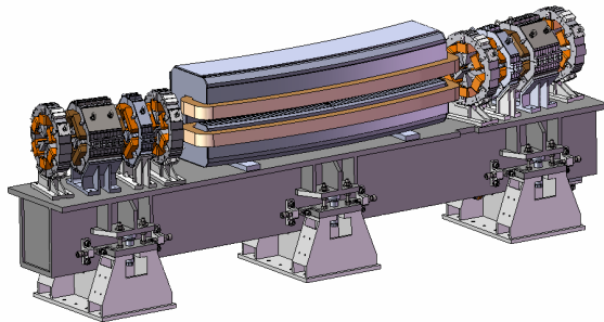
Figure 4: Half cell SESAME magnet-girder assembly.
