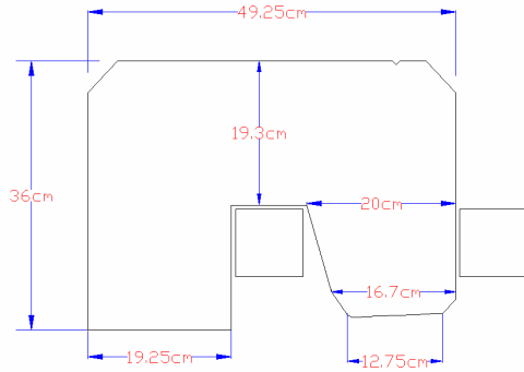
Figure 3: SESAME bending magnet lamina.
