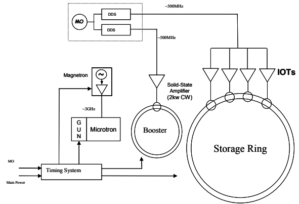
Figure5: Block diagram of SESAME RF system
