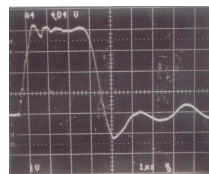
Figure 2: The modulator pulse current that we measured (left) compared to the one measured at BESSY I in 1998(right).
