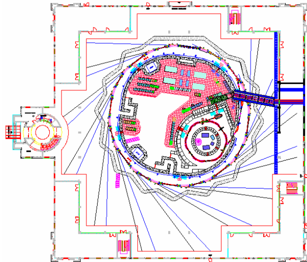
Figure 6: SESAME layout in the experimental hall.
